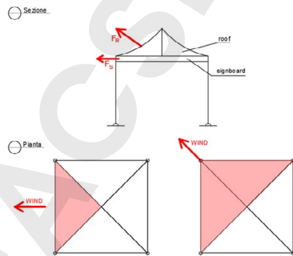
Figure 1 Force application
